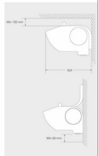
Fig. 1: Distance minimale
