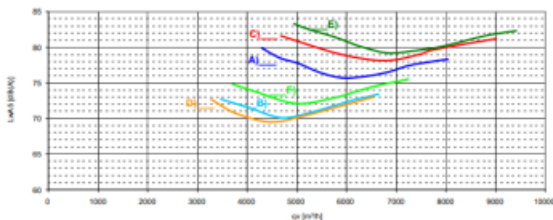
2. Diagramme / Chart 2 - Volumestrom / Airflow - Abstrahl / Acoustic
