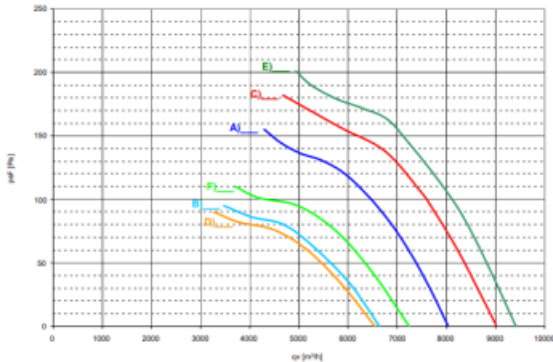
2. Diagramme / Chart 2 - Volumestrom / Airflow - Abstrahl / Acoustic
